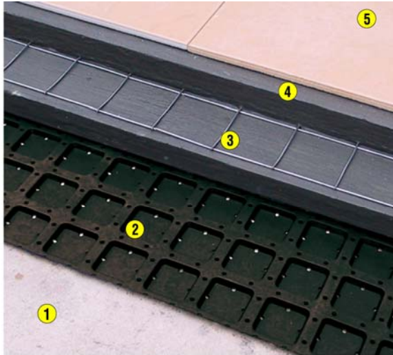
1 Floor Slab 2 VersiDrain® 6P 3 Reinforcing Mesh 4 Cement and Sand Screed / Concrete 5 Floor tile
